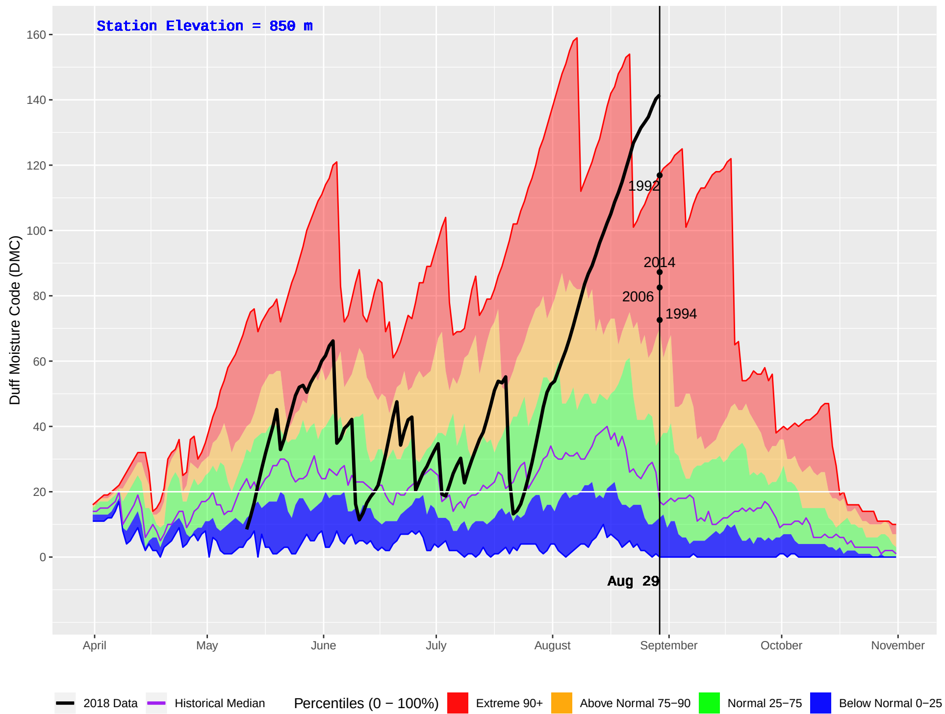
NORTH CHILCO (159) : Historical (1972–2016) and Current (2018) Daily Duff Moisture Code (DMC)
