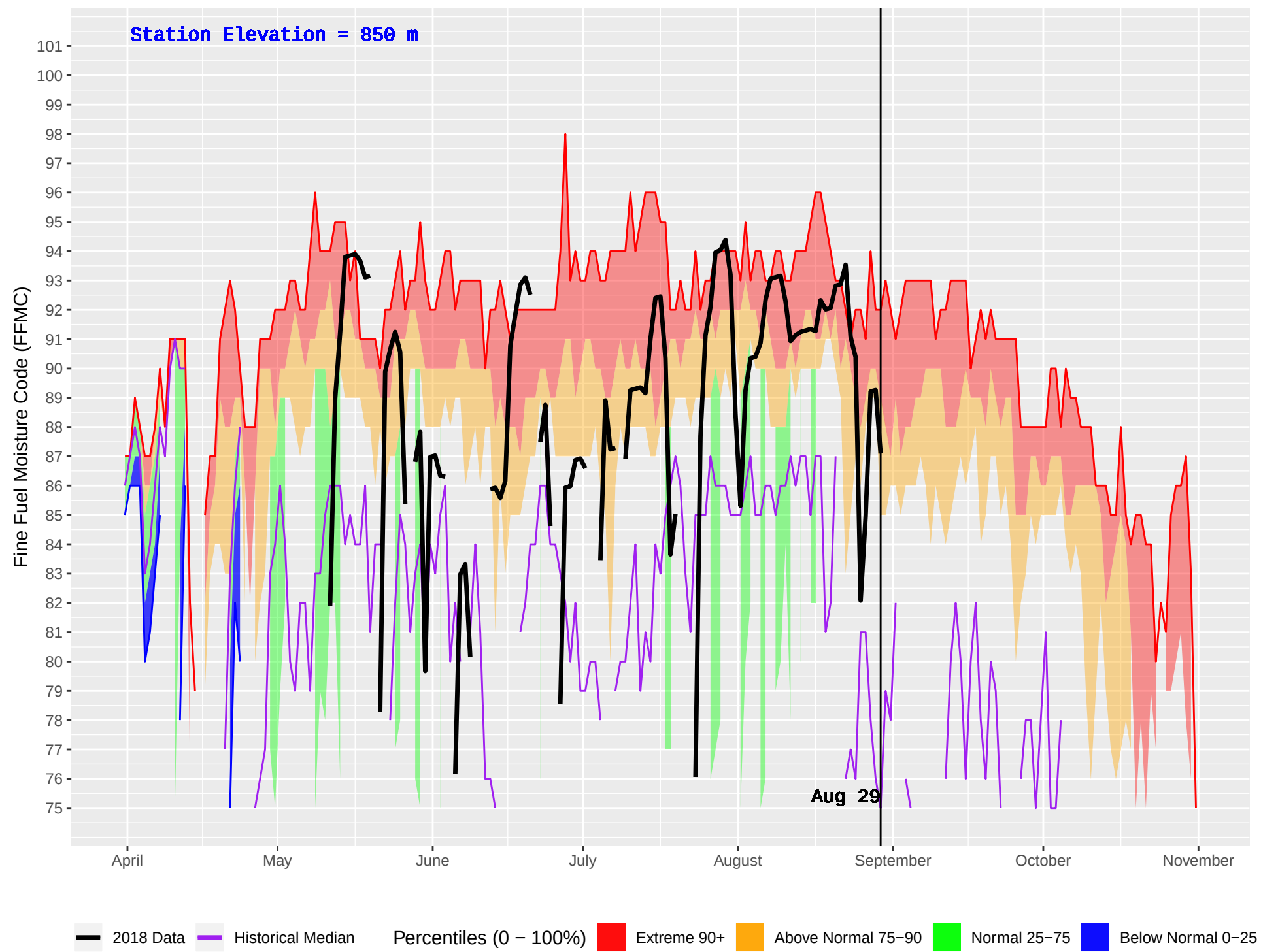
NORTH CHILCO (159) : Historical (1972–2016) and Current (2018) Daily Fine Fuel Moisture Code (FFMC)
