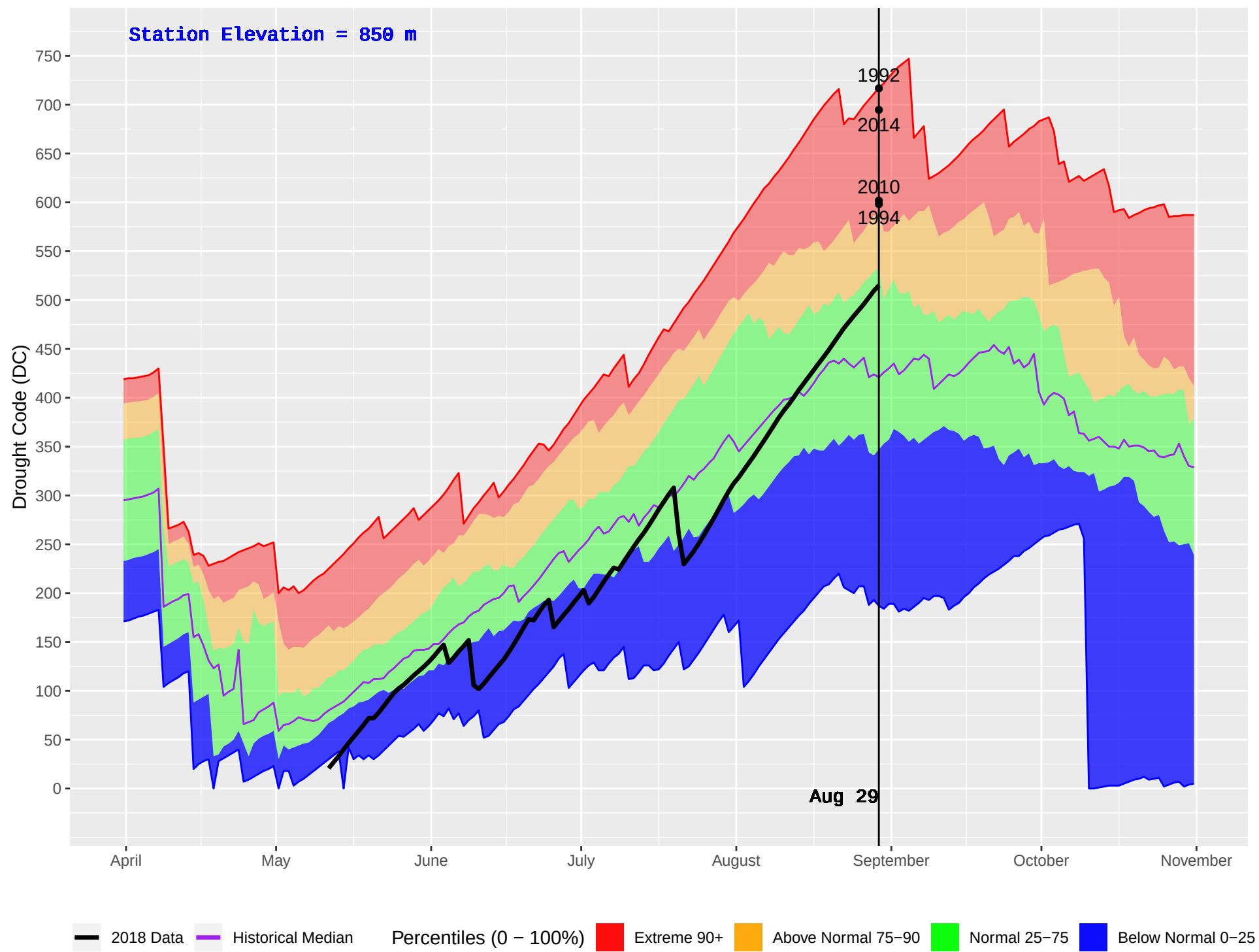
NORTH CHILCO (159) : Historical (1972–2016) and Current (2018) Daily Drought Code (DC)
