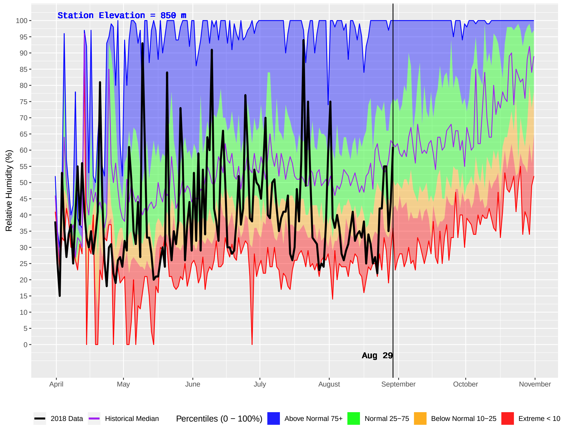
NORTH CHILCO (159) : Historical (1972–2016) and Current (2018) Daily Relative Humidity
