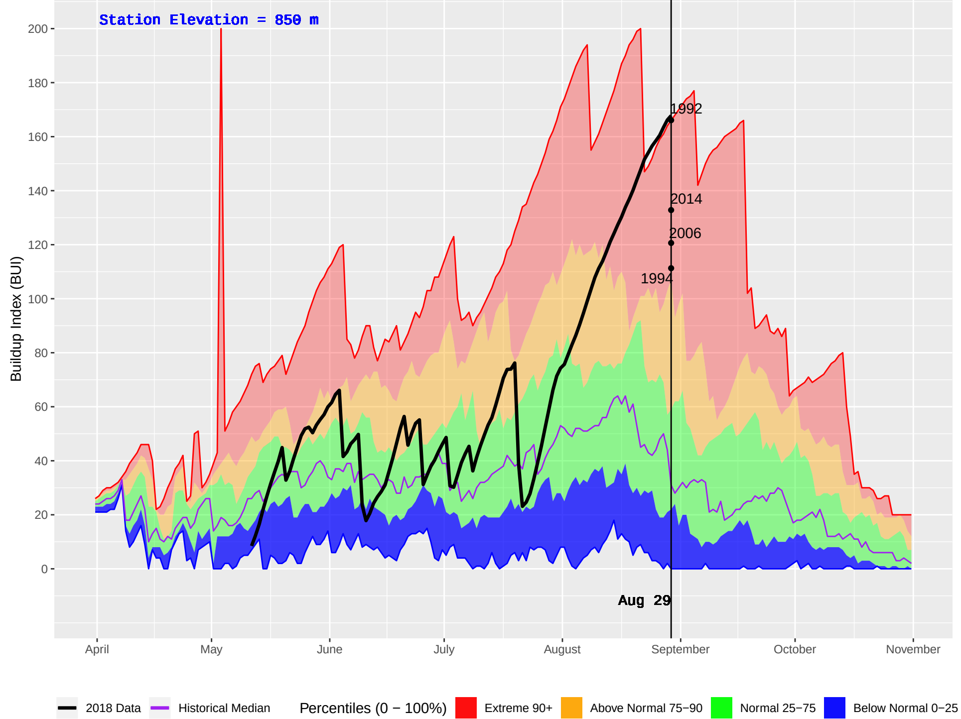
NORTH CHILCO (159) : Historical (1972–2016) and Current (2018) Daily Buildup Index (BUI)
