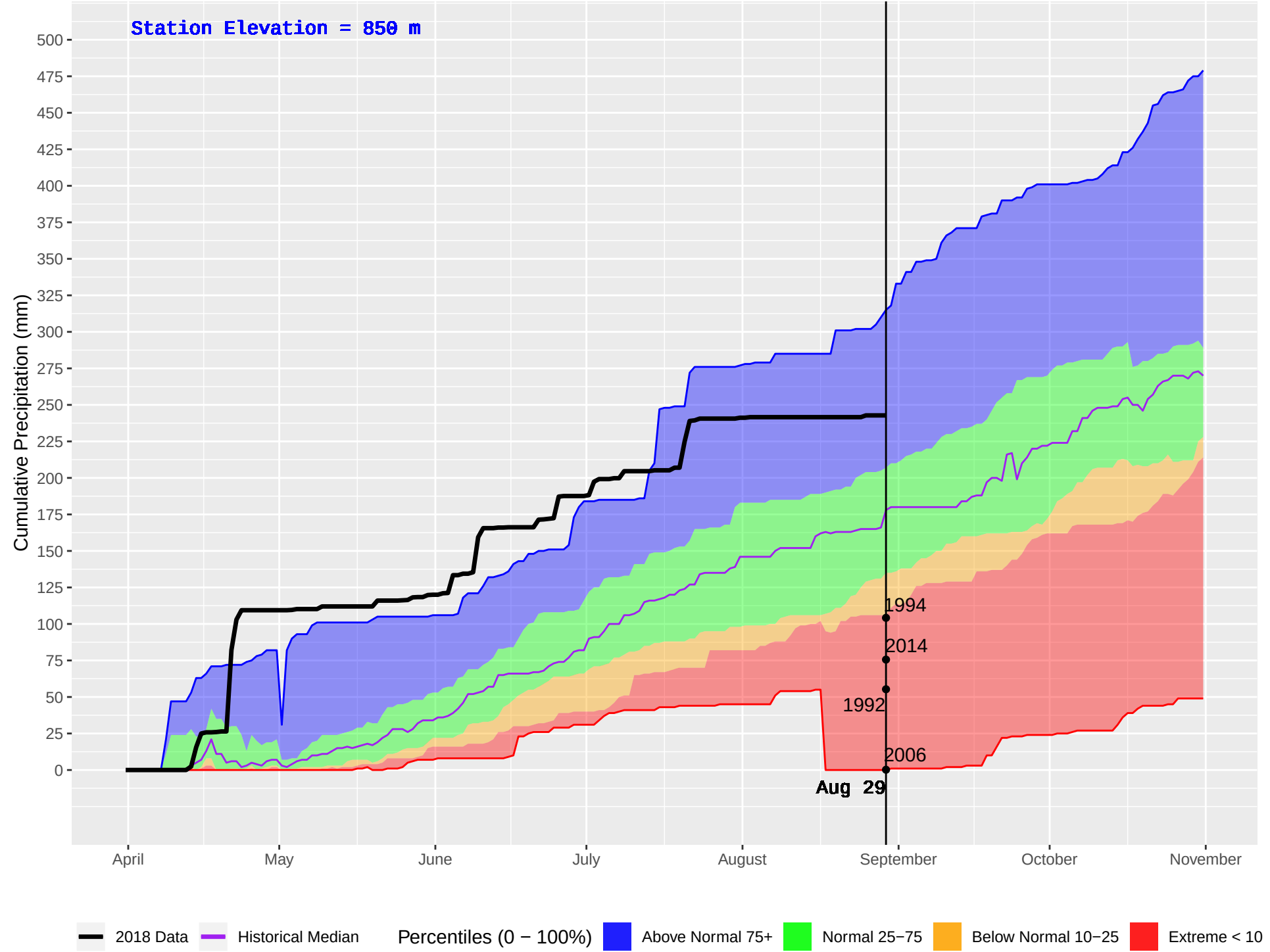
NORTH CHILCO (159) : Historical (1972–2016) and Current (2018) Daily Cumulative Precipitation
